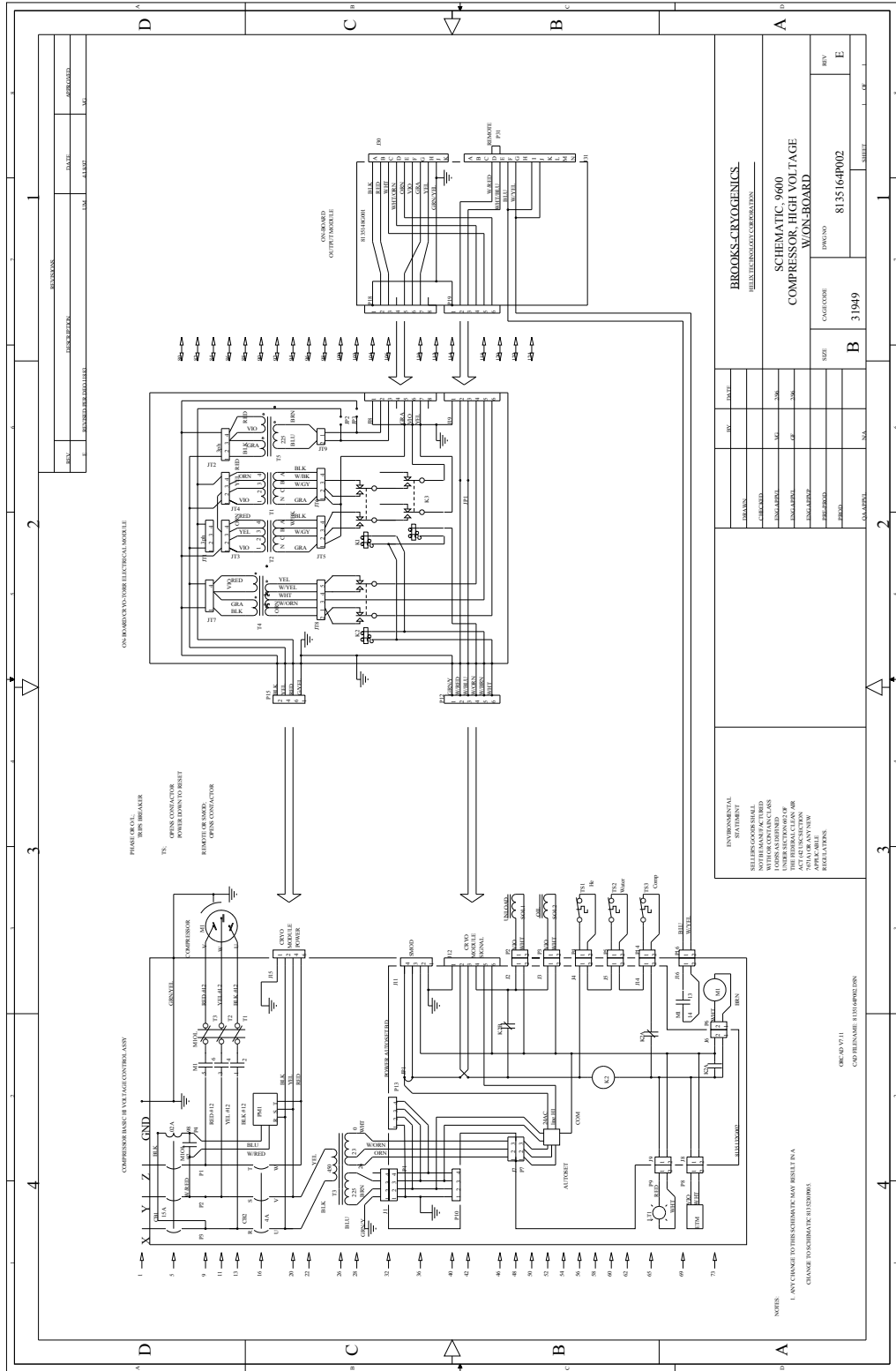
Figure D-1: 9600 High Voltage Compressor
